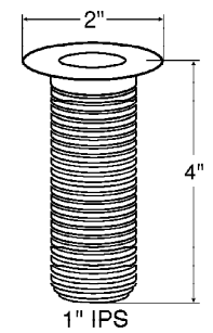
HEAVY CAST DRAIN ASSEMBLY FOR BAR SINK - CHROME
