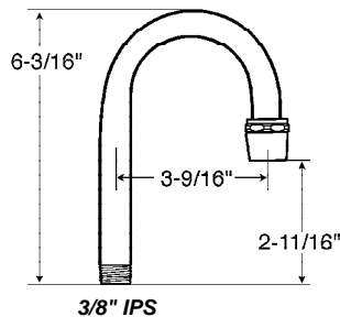
BAR SINK SPOUT # 2356
