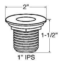
HEAVY CAST DRAIN ASSEMBLY FOR BAR SINK - CHROME
